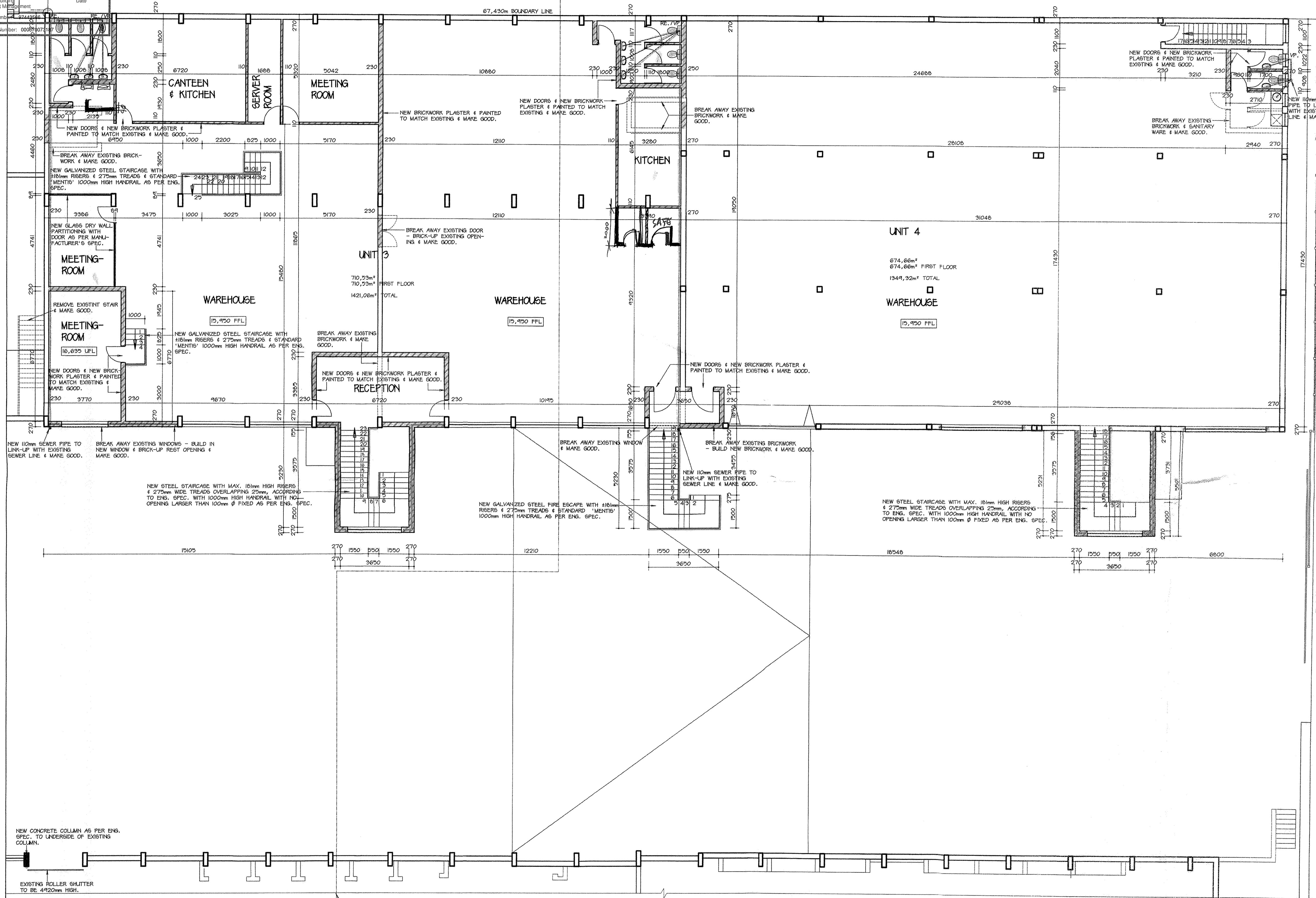
BLOCK 4 - PART FIRST STOREY PLAN 1 : 100
