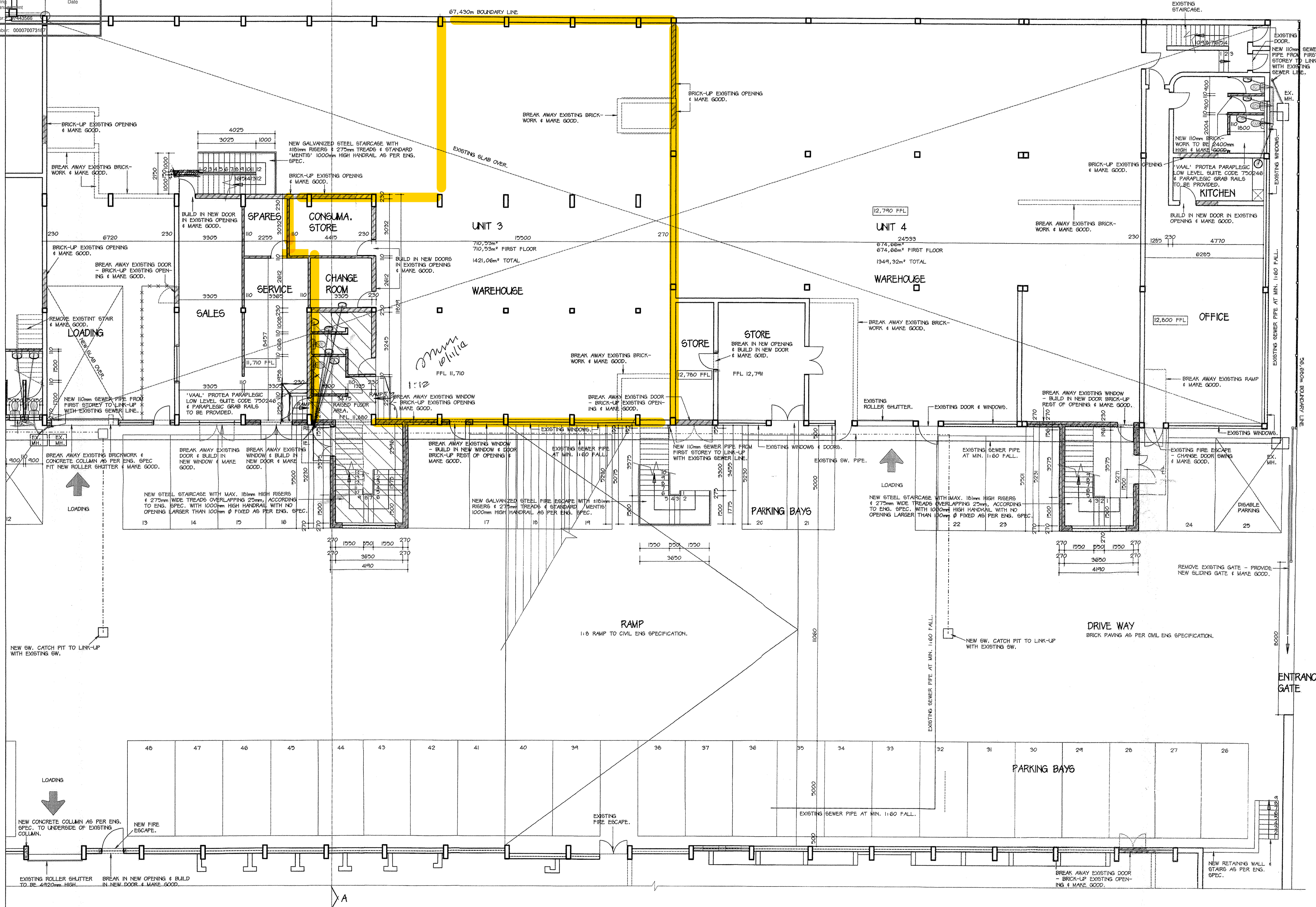
BLOCK 4 - PART GROUND STOREY PLAN 1 : 100
